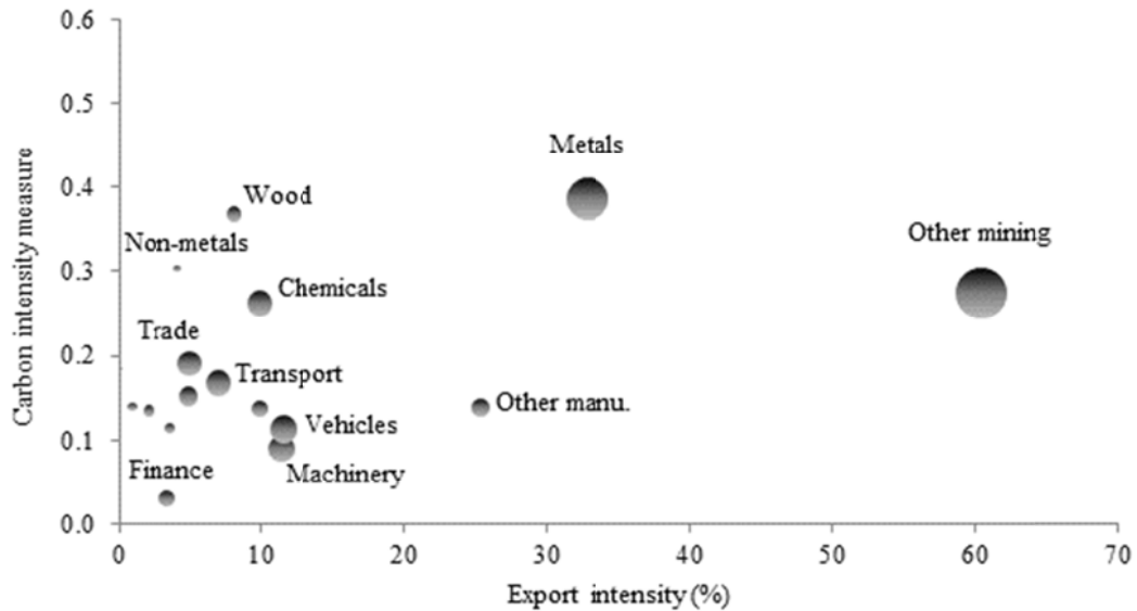
Figure 2: Carbon and export intensities for aggregate products (2005)
