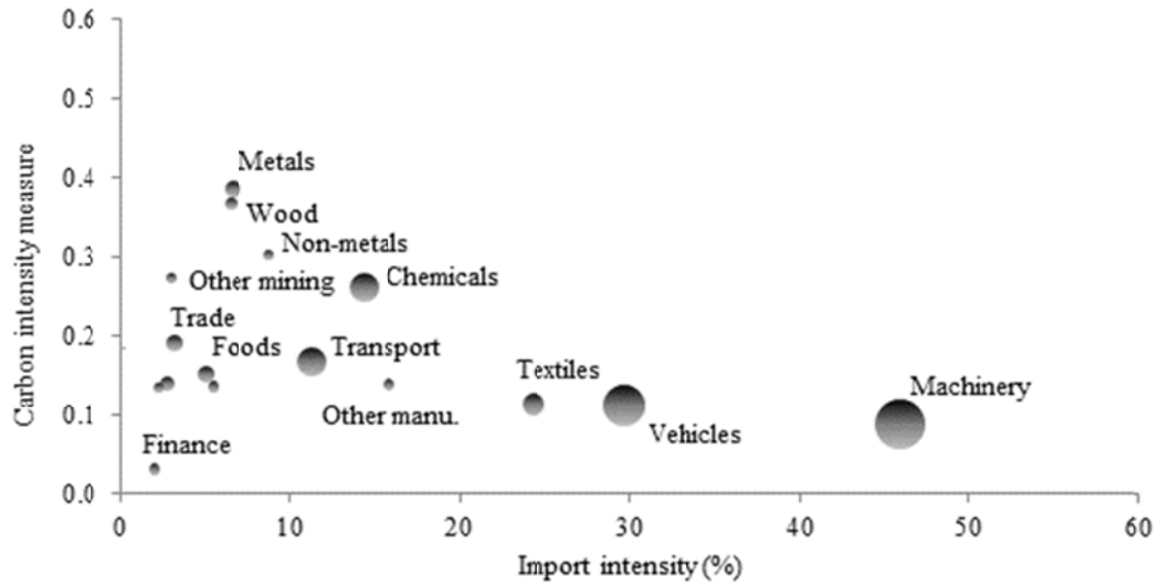
Figure 3: Carbon and import intensities for aggregate products (2005)
