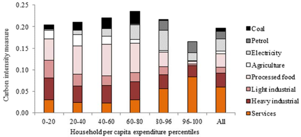
Figure 1: Decomposing the carbon intensity of household consumption (2005)
